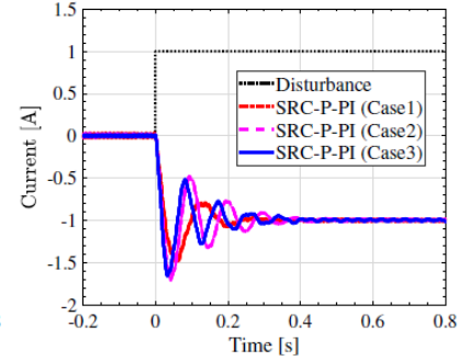
(b) Disturbance and feedback current.
