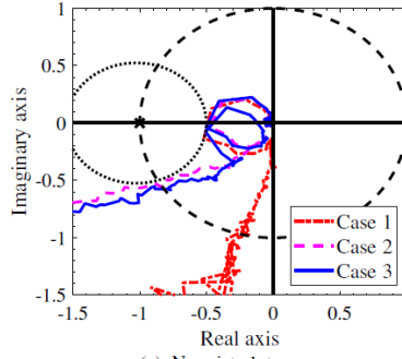
Fig. 7. Design results of the velocity loop (SRC-P-PI control).
