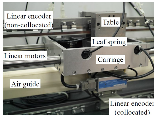
Fig. 1. High-precision positioning stage.
