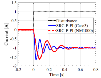
(b) Disturbance and feedback current.
