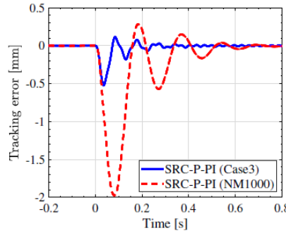
(a) Tracking error.
