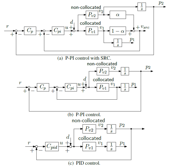
Fig. 5. Block diagrams of the compared controller configurations.
