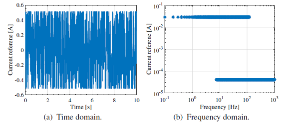
Fig. 3. Current input for system identification (data set 1: 0.1 – 120 Hz).
