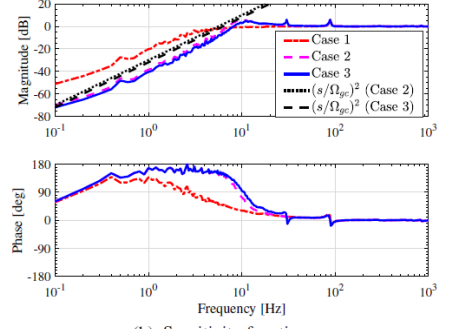
Fig. 7. Design results of the velocity loop (SRC-P-PI control).
